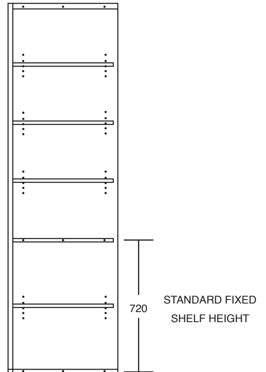
CABINET CONSTRUCTION – STANDARD BROOM
