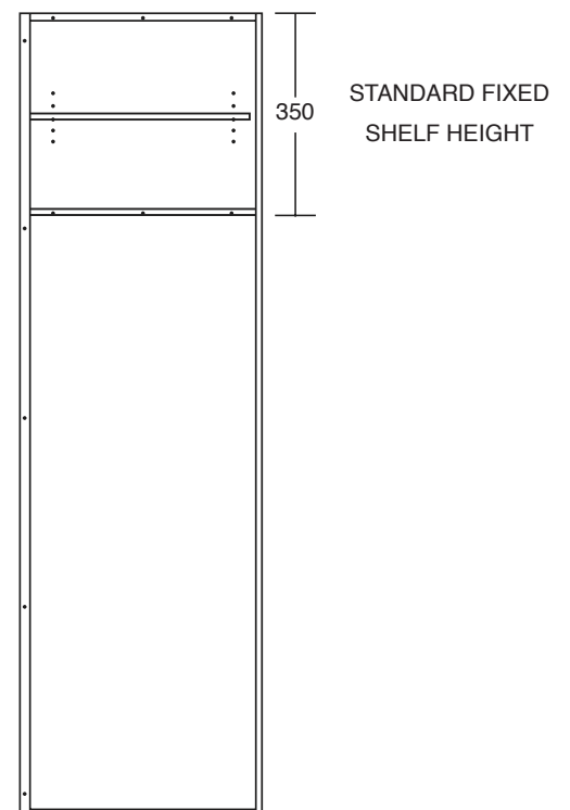
CABINET CONSTRUCTION – STANDARD BROOM
