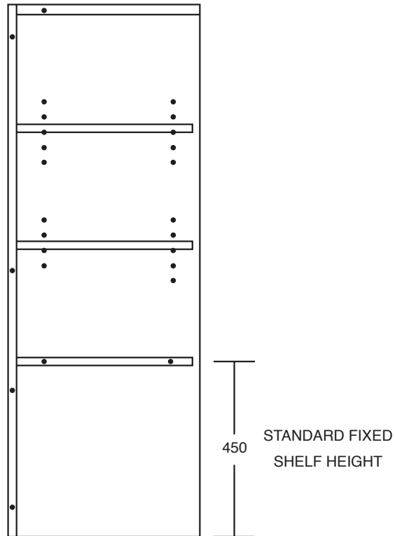
CABINET CONSTRUCTION – STANDARD CORNER PANTRY
