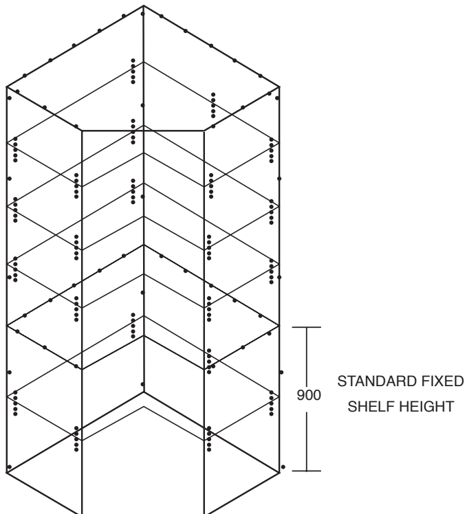
CABINET CONSTRUCTION – STANDARD CORNER PANTRY
